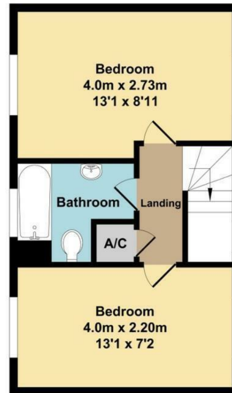
1st Floor Approx. Floor Area 27.92 Sq.M. (300 Sq.Ft.)
